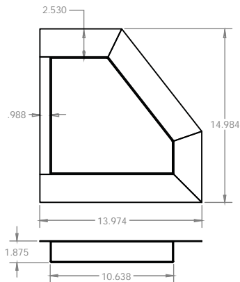
Ash Cup Dimensions
